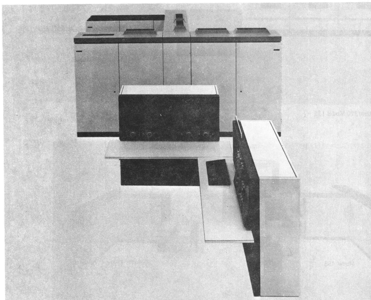
Figure 1-4. System/370 Model 168
