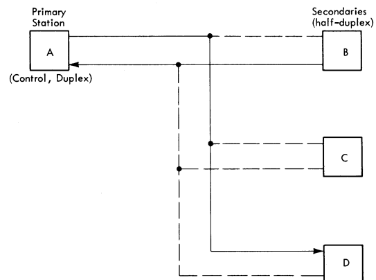
C. "Multi-multipoint" Duplex Data Link (A "talks" to D while it is "listening" to B)
