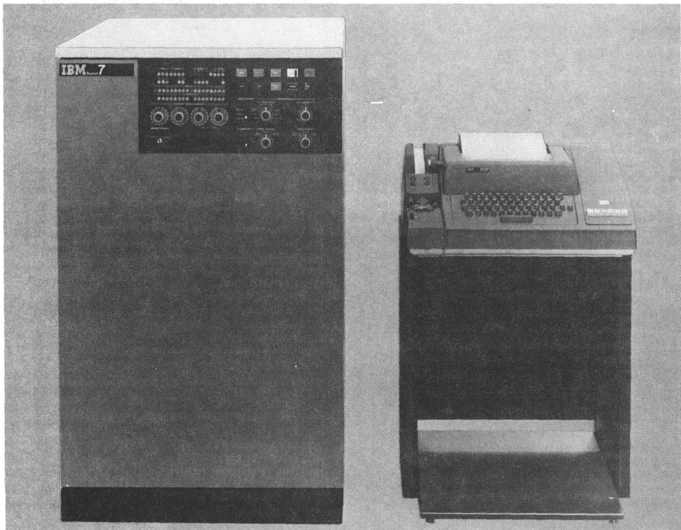
Figure 8-40. IBM System/7
