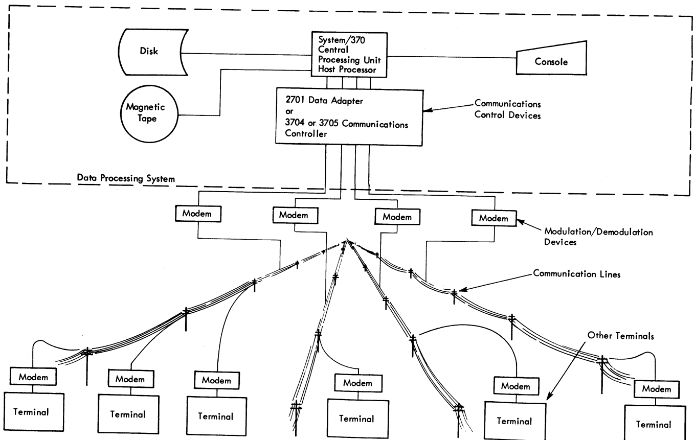
Figure 5-1. A Teleprocessing Network
