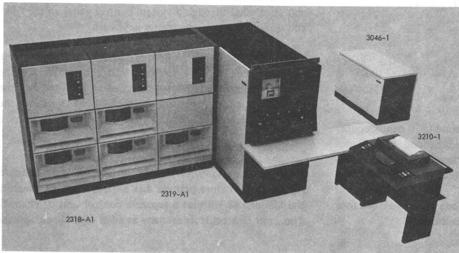
Figure 6-3. IBM System/370 Model 135 with IBM 2318 and 2319 Disk Storage, IBM 3210 Console Printer-Keyboards, and IBM 3046 Power Unit
